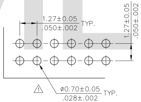
Recommended P.C. Boarded Layout
